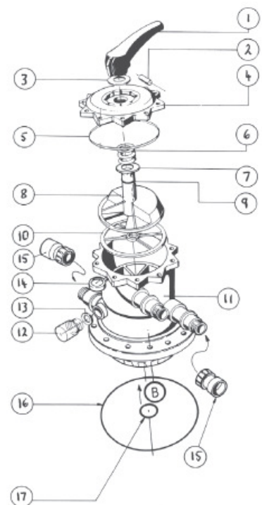
Backwash Valves
